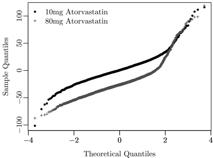
Figure 2.2 Normal probability (Q-Q) plot of change in LDL at 3 months by treatment in the TNT study.
